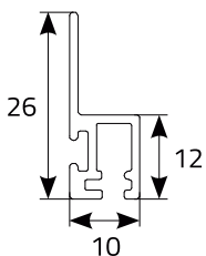
unteres "H"-Profil (Standard)
